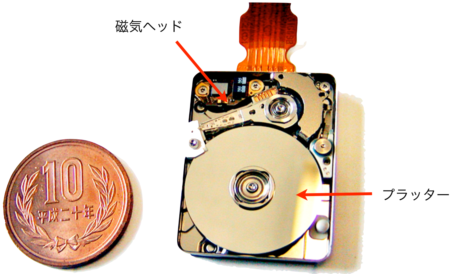
0.85inch, 4GB (2005)
